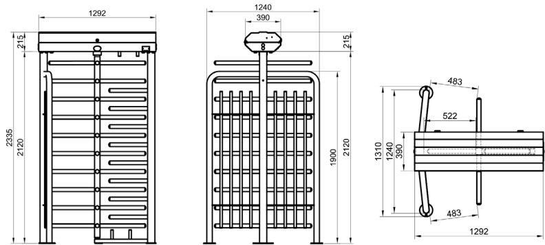
Dimensions (mm)
